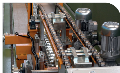
Multi-purpose patented trolley for plates' moving and cloths washing system, with integrated maintenance hoist
